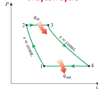
Brayton cycle
